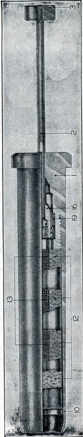
FIGURE 7.—Friction primer, M1914.
