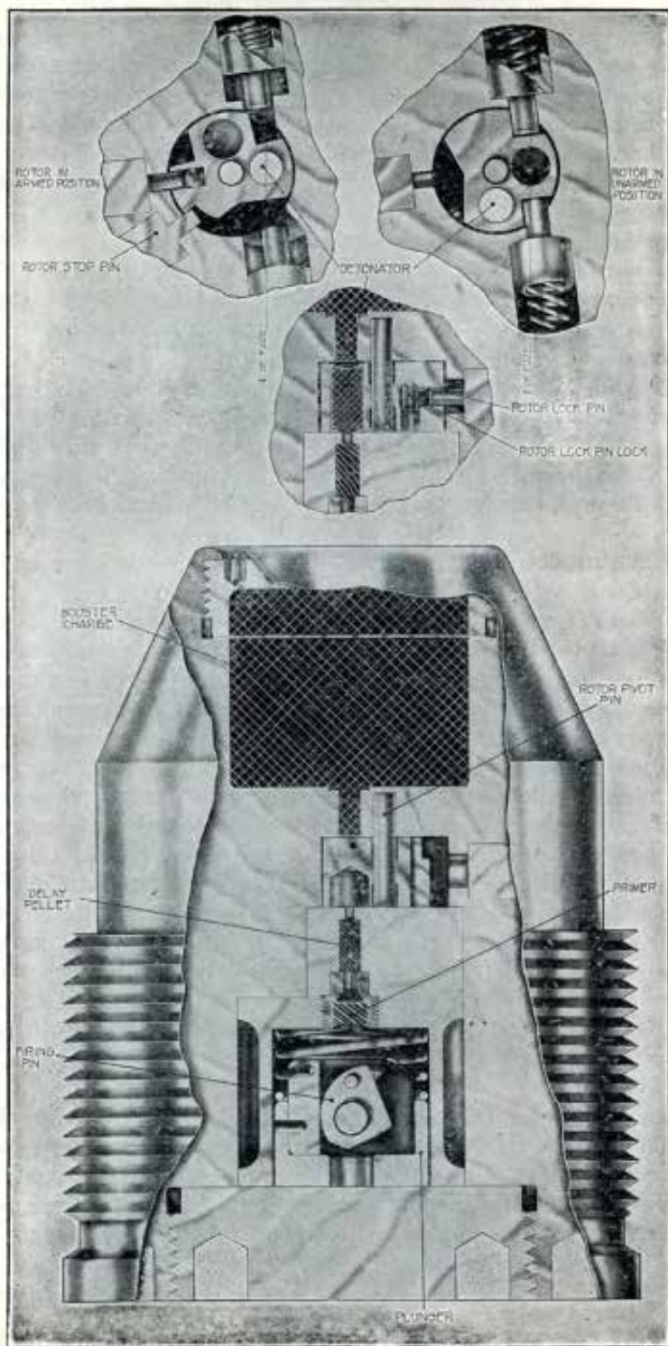
FIGURE 13.—Base Detonating Fuse, Mk. X.
