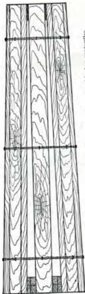
FIGURE 35.—Crate for shipping projectiles.
