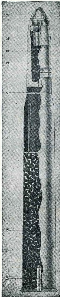
FIGURE 1.—Complete round 3-inch antiaircraft ammunition.
