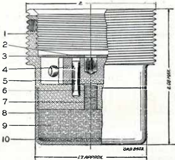
FIGURE 23.—Booster, M20.
