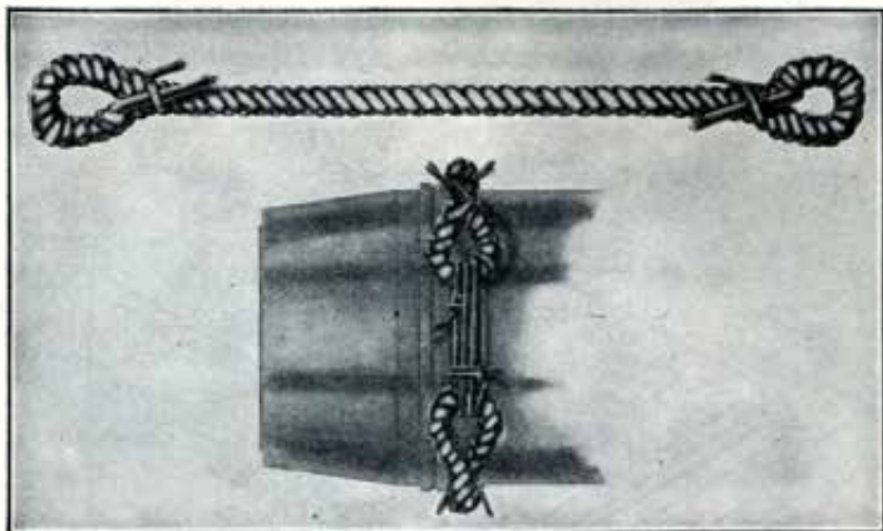
FIGURE 36.—Rope grommet.
