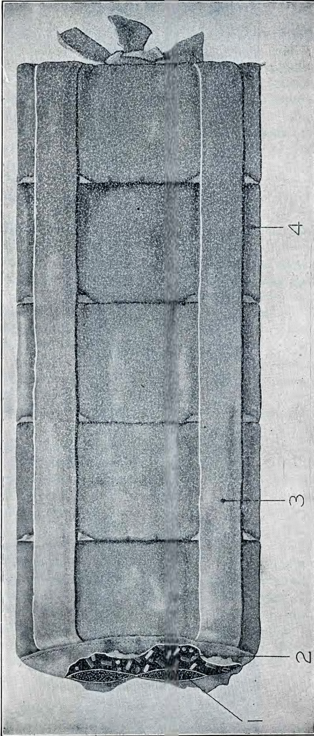
FIGURE 5.—240-mm howitzer propelling charge (alliquot part type).
