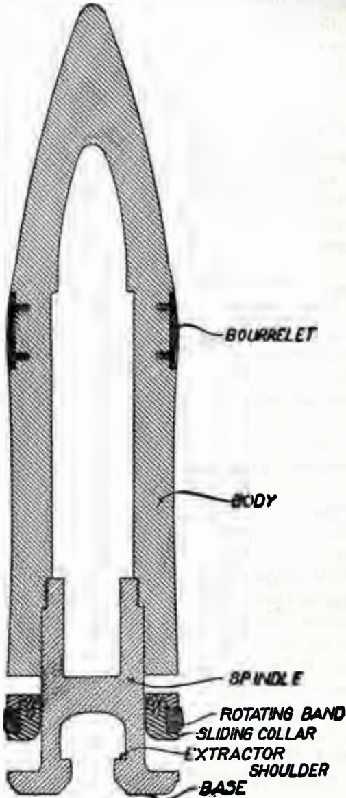
FIGURE 31.—Dummy projectile (new type).
