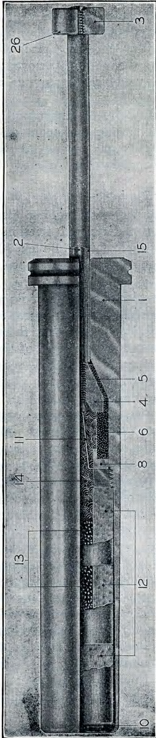
FIGURE 8.—Electric primer.
