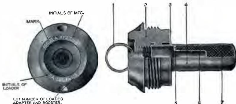
FIGURE 20.—Adapter and booster, Mk. III-A M2.
