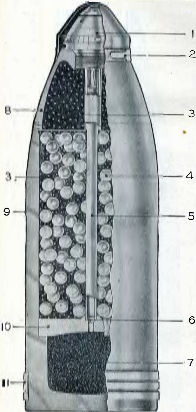
FIGURE 29.—155-mm shrapnel, Mk. I
