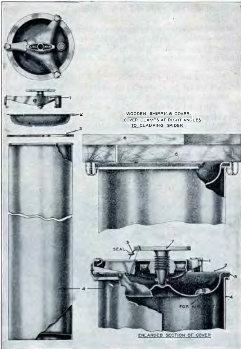
FIGURE 39.—Storage case for propelling charge.
