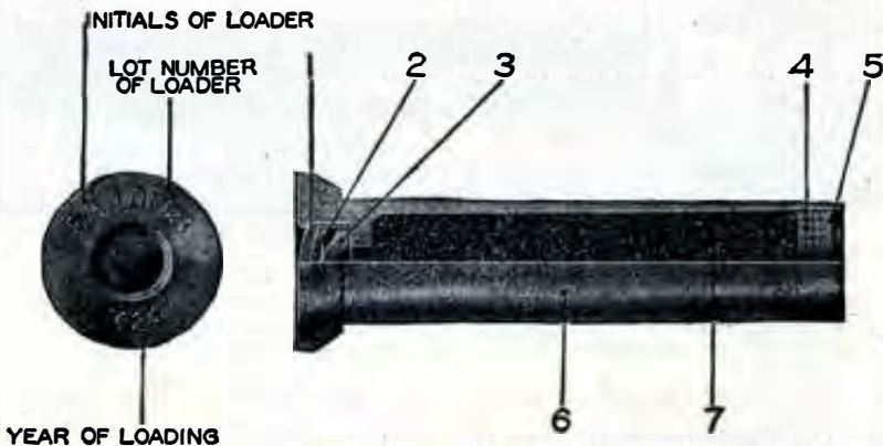
FIGURE 9.—21-grain percussion primer, Mk. II-A.
