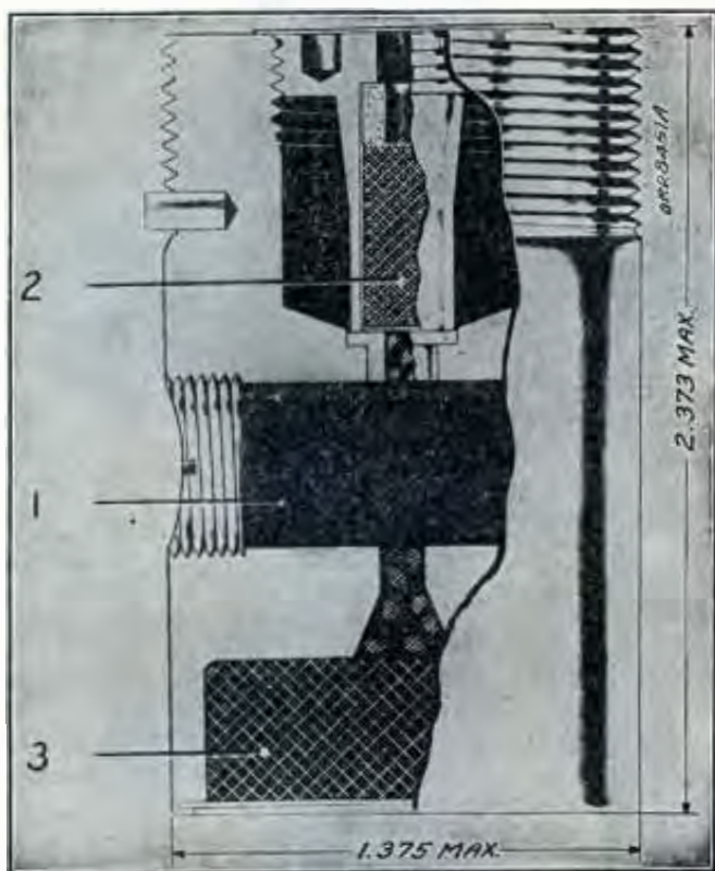
FIGURE 22.—Antiaircraft booster, Mk. X.
