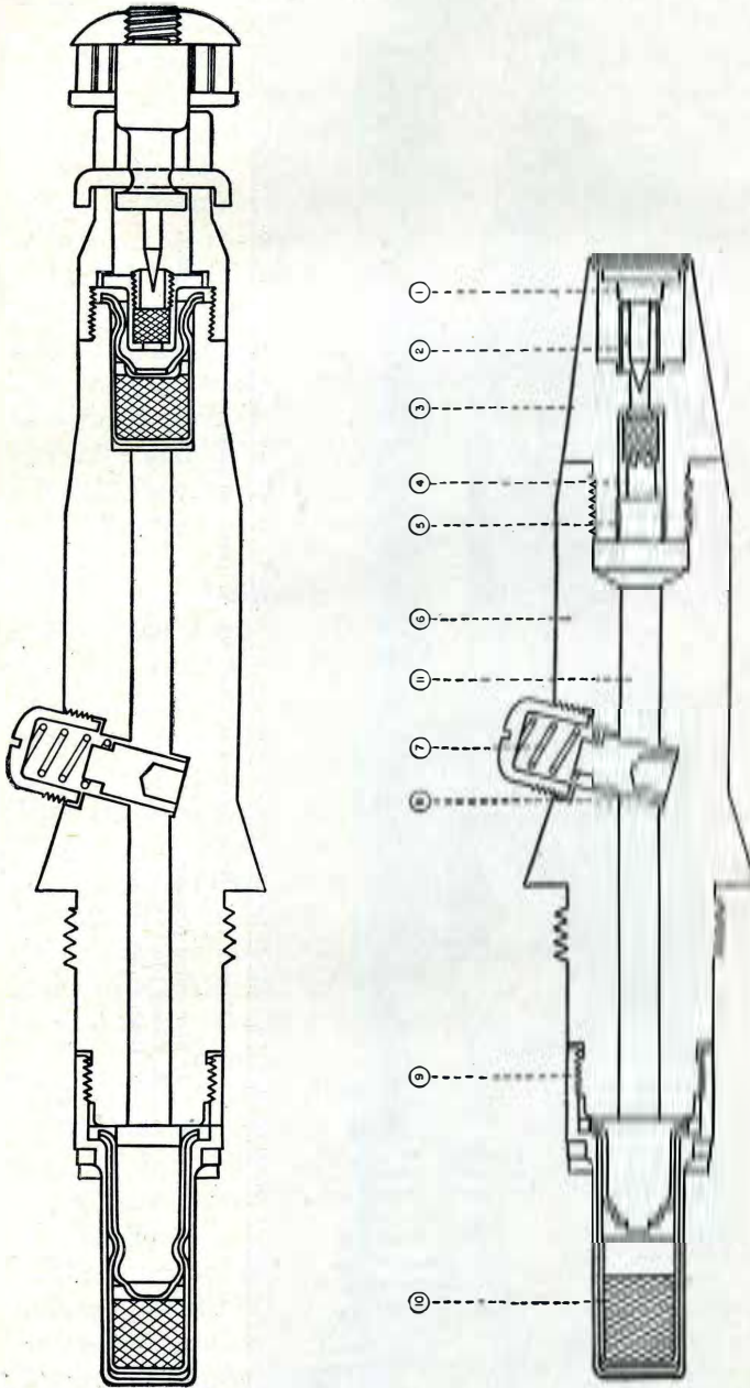
FIGURE 15.—Point detonating fuze, M46.
