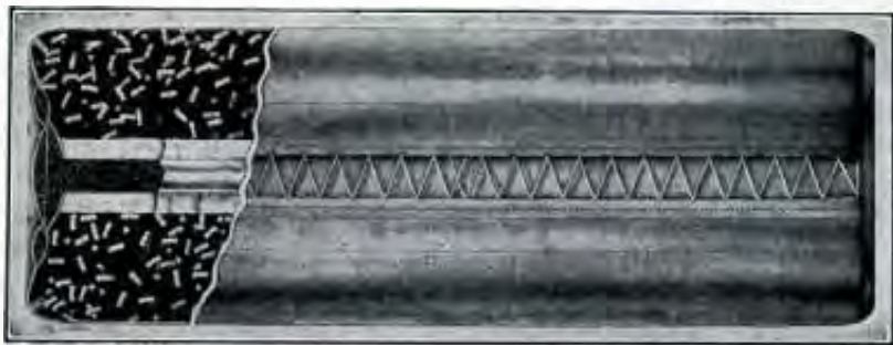
FIGURE 3.—Single-section propelling charge.
