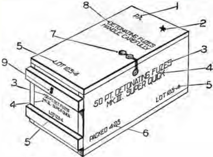
FIGURE 38.—Packing box for point detonating fuzes.
