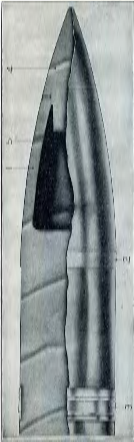
FIGURE 30.—Target-practice projectile.
