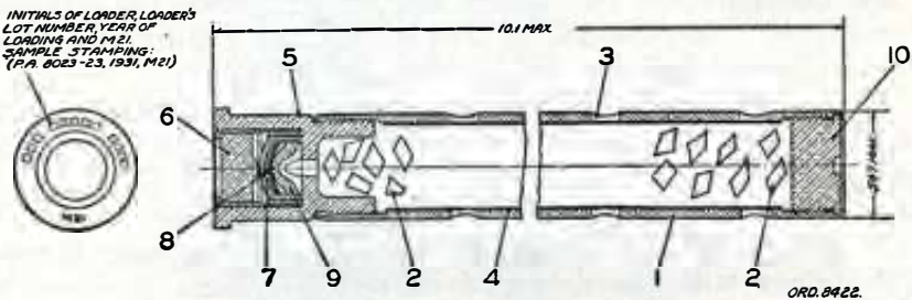
FIGURE 11.—Primer, percussion, M21.
