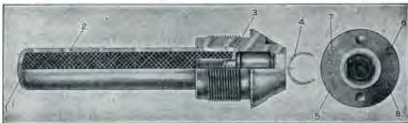
FIGURE 19.—Adapter and booster, Mk. II-A.
