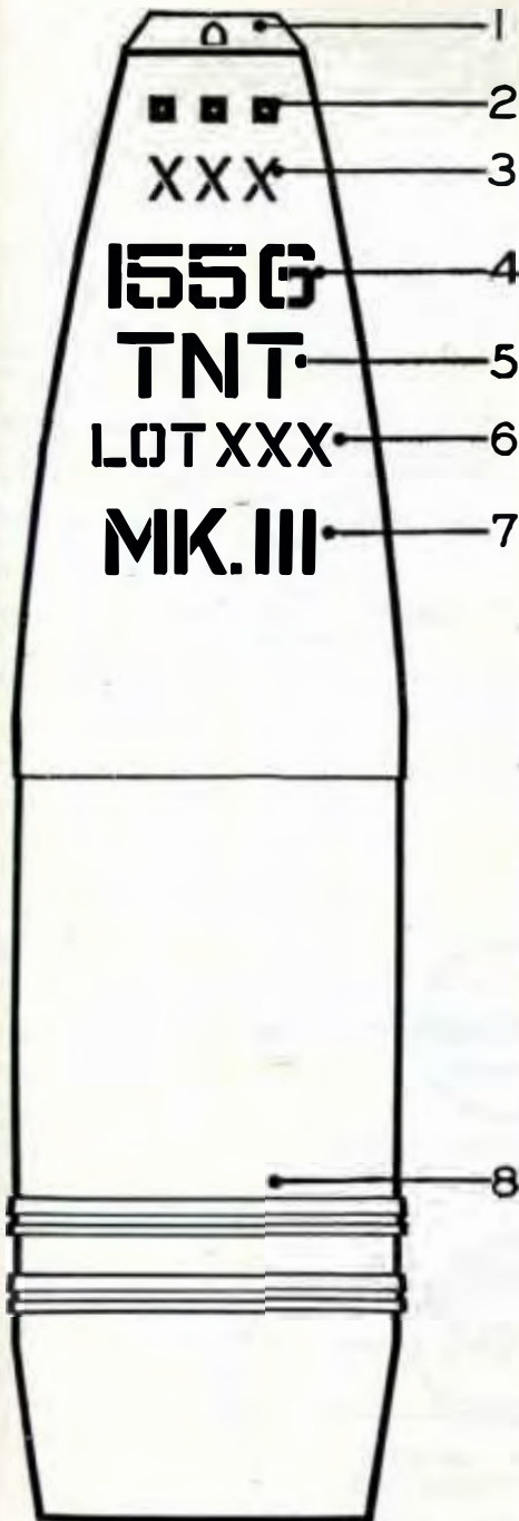
FIGURE 33.—Marking for high-explosive shell for 155-mm gun, 6-inch gun, 8-inch gun or howitzer, and 240-mm howitzer.
