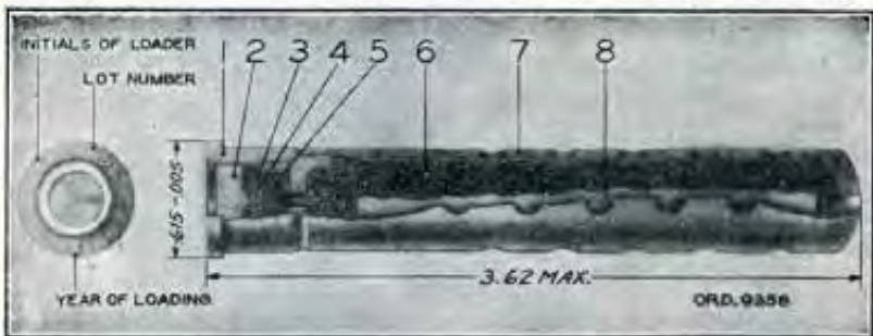
FIGURE 10.—Primer, percussion, 100-grain, M1.
