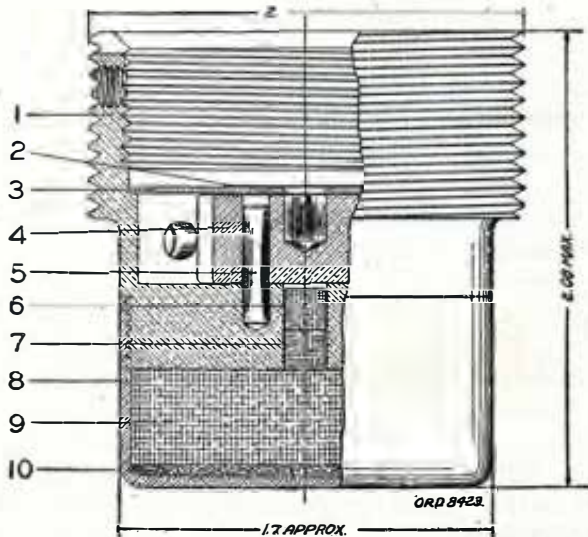
FIGURE 23.—Booster, M20.
