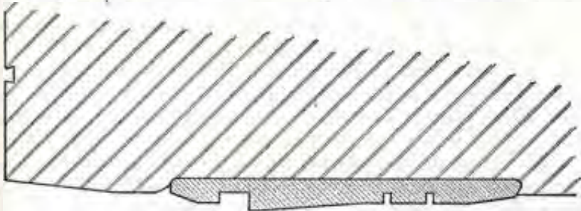
FIGURE 25.—Rotating band.
