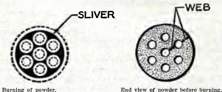
FIGURE 2.—Grain of smokeless powder.
