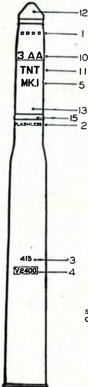
FIGURE 34.—Marking for fixed ammunition for antiaircraft guns.
