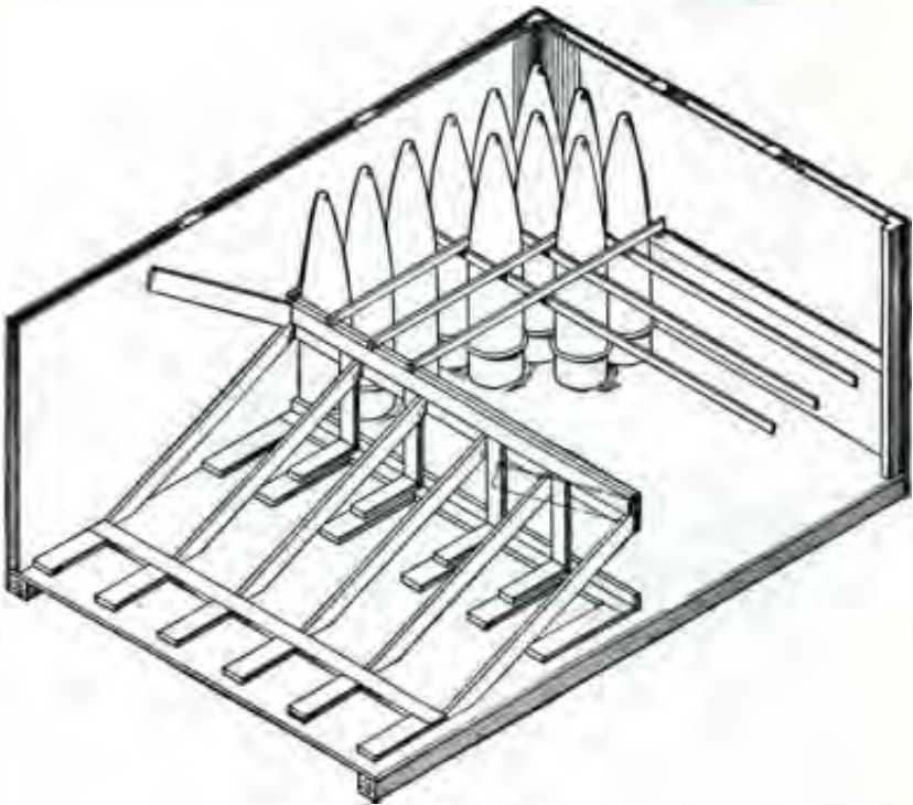
FIGURE 37.—Method of packing projectiles in freight cars.
