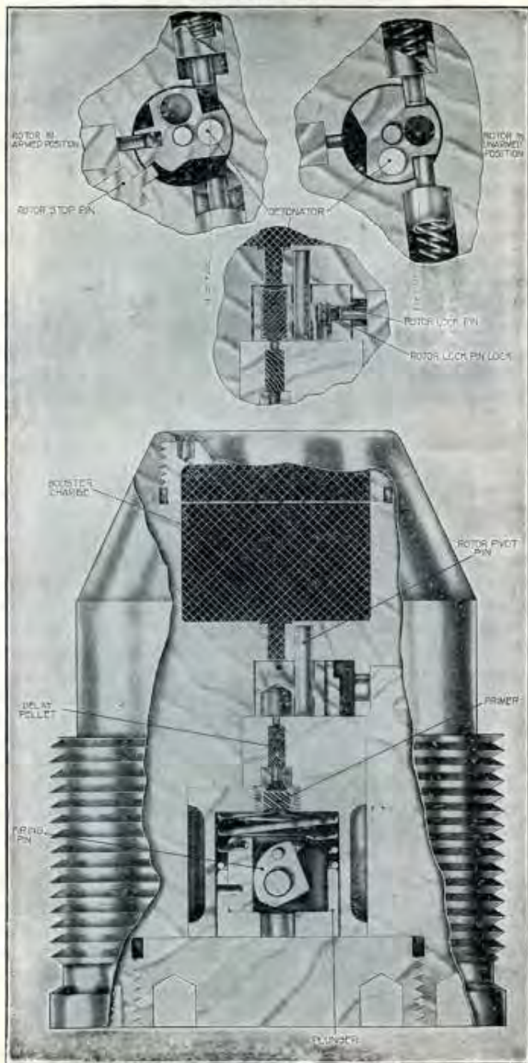
FIGURE 13.—Base Detonating Fuze, Mk. X.
