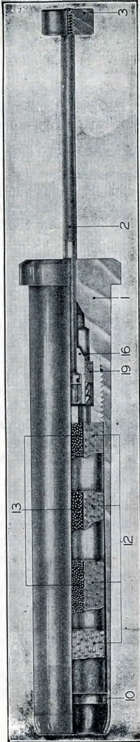
FIGURE 7.—Friction primer, M1914.
