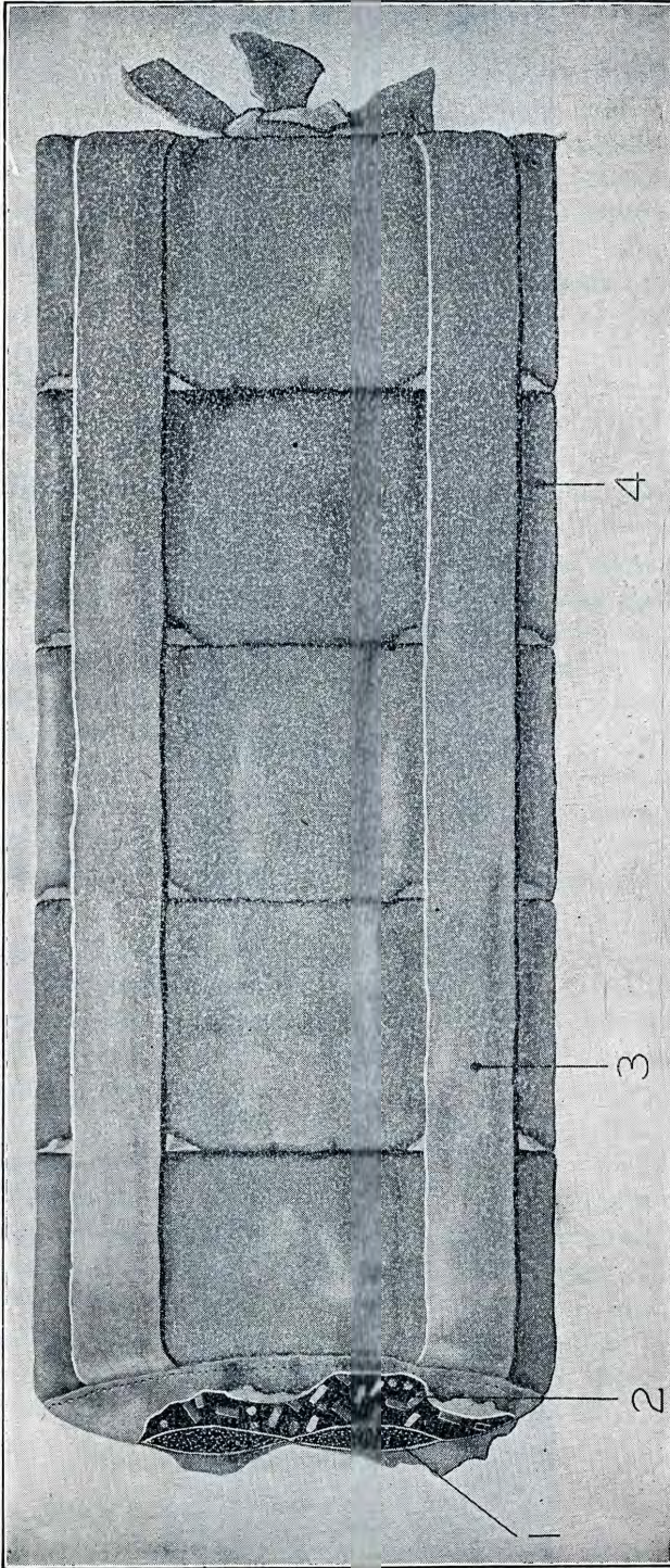
FIGURE 5.—240-mm howitzer propelling charge (aliquot part type).
