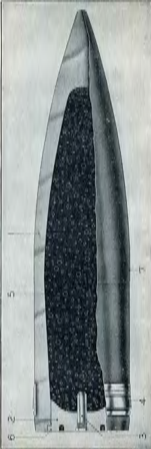
FIGURE 28.—High-explosive shell.
