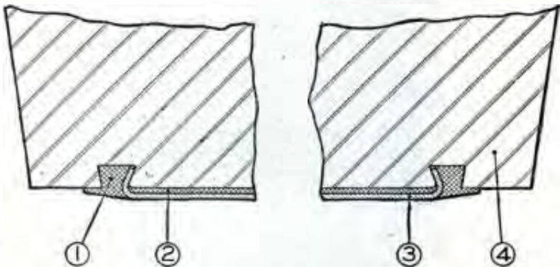
FIGURE 26.—Base cover.
