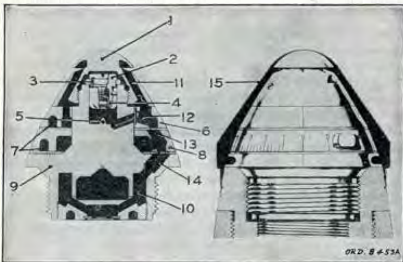
FIGURE 17.—Anti-aircraft time fuze, Mk. III.
