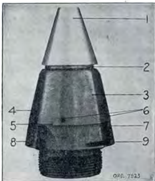
FIGURE 18.—Fuze, mechanical time, M43. (Fuze set for 29 \frac{3}{4} seconds.)
