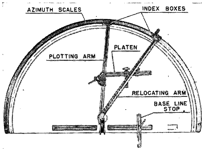
FIGURE 61.—Plotting and relocating board M1923 (Clove).
