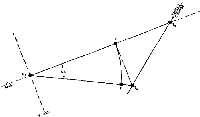
FIGURE 193.—Range prediction, incoming target.
