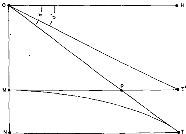
FIGURE 24.—Effect of curvature of earth on line of sight.
