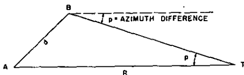
FIGURE 10.—Parallax diagram for general formula.
