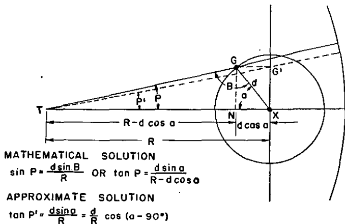
FIGURE 166.—Parallax problem No. 1.
