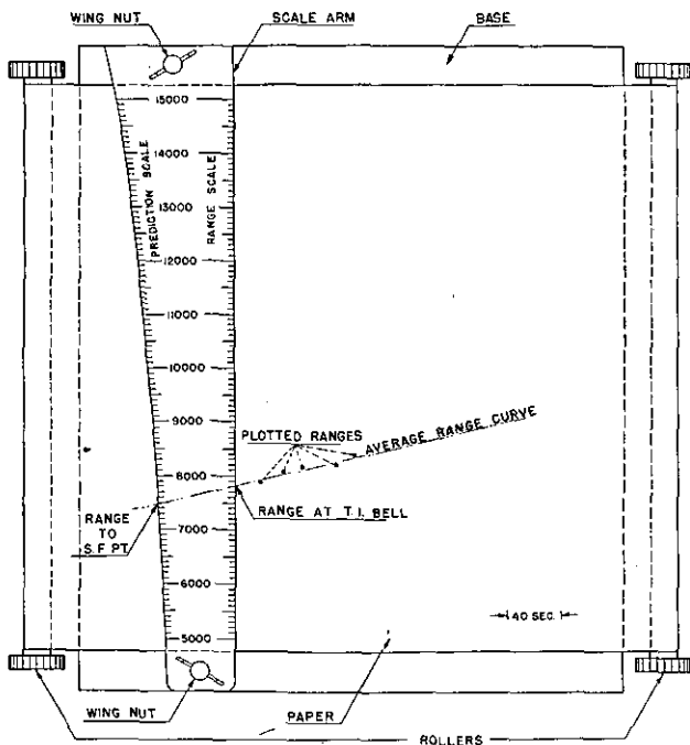
FIGURE 50.—Typical time-range board.
