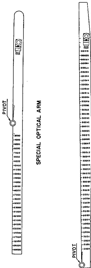
STANDARD OPTICAL ARM FIGURE 59.—A comparison of the standard and special optical station arms.
