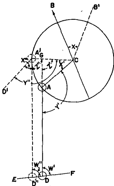
FIGURE 111.—Theory of aiming rule.
