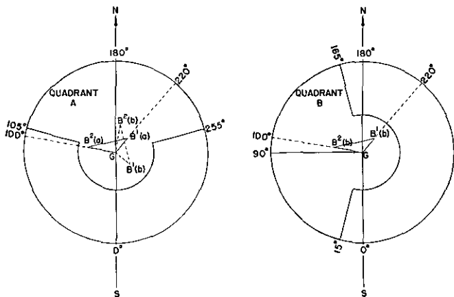
FIGURE 52.—Arrangement of quadrant positions on 110^\circ plotting board.
