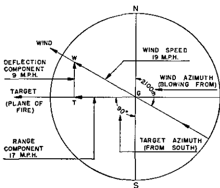
FIGURE 68.—Wind component indicator.
